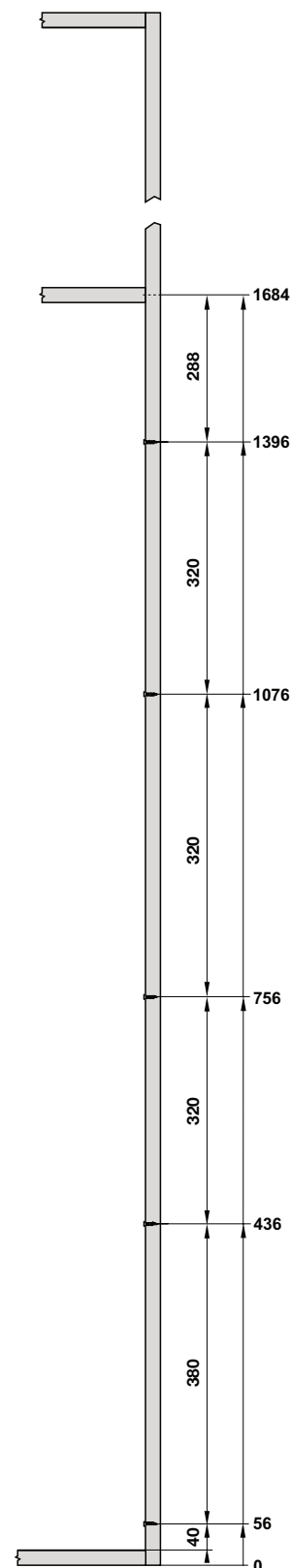
Cabinet drilling
