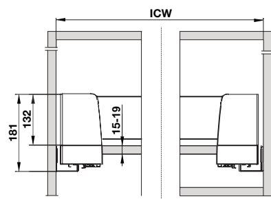
Bottom panel drilling dimensions
