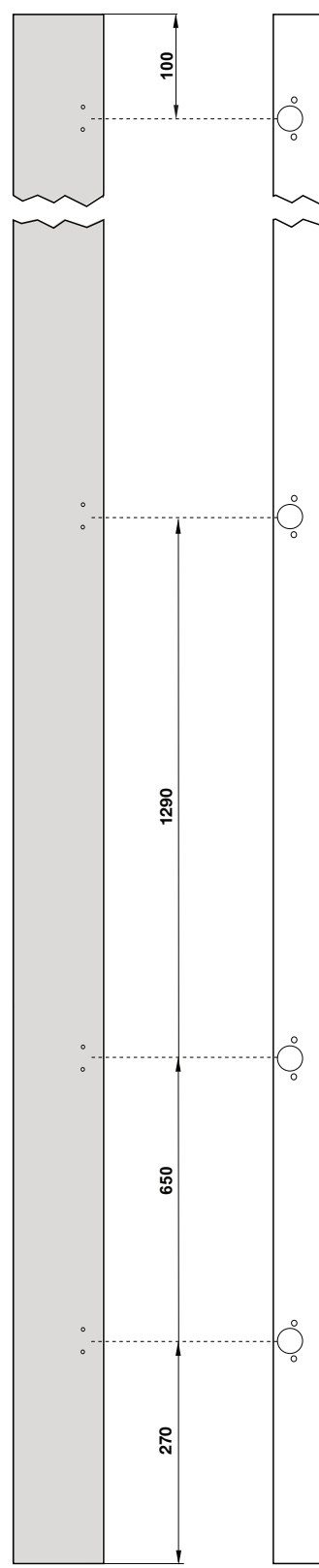
Door panel drilling
