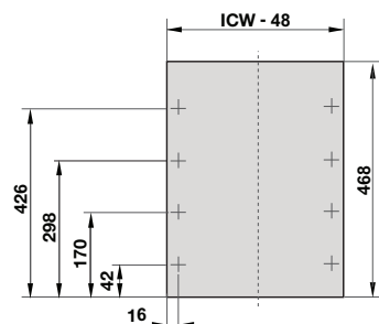
Bottom panel drilling dimensions
